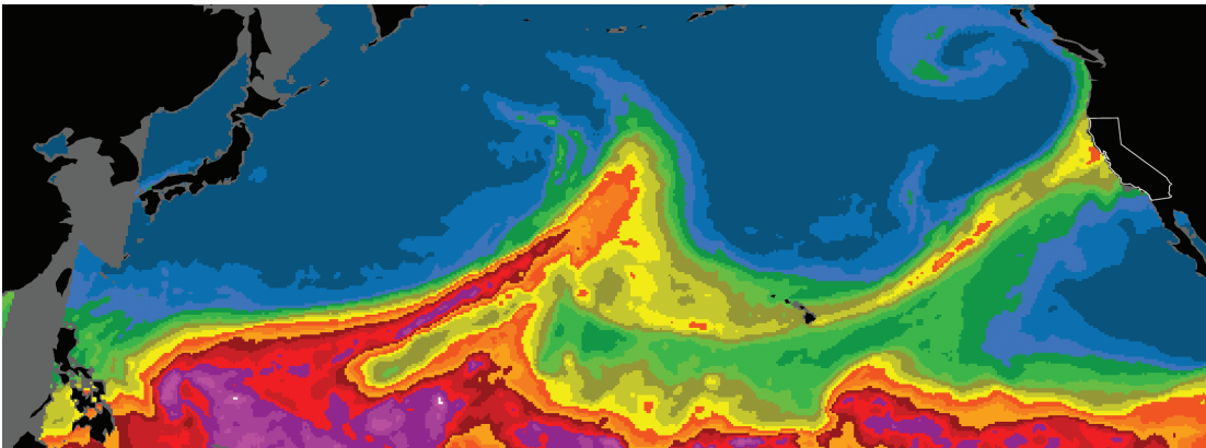
Satellite image of atmospheric river reaching West Coast. Atmospheric river storms — storms fueled by concentrated streams of water vapor from the Pacific Ocean — are responsible for most episodes of major West Coast flooding. The HMT's efforts in California were responsible for identifying this storm type and its importance for flood management and water supplies. NOAA figure
